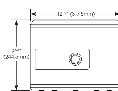
11Qt - FRONT VIEW
