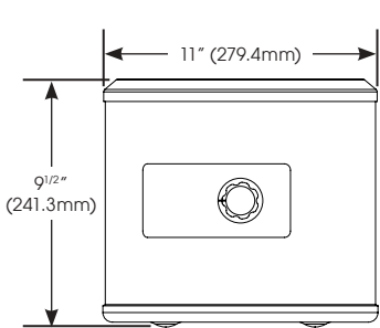
7Qt - FRONT VIEW
