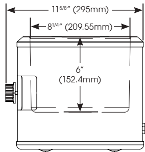
7Qt - SIDE VIEW
