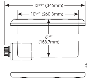
11Qt - SIDE VIEW
