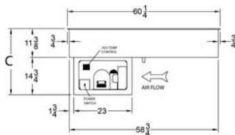
FRONT ELEVATION (OPERATOR SIDE)
