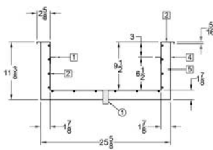
SECTION VIEW SCALE: 1"=1'
