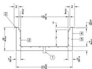
SECTION VIEW
