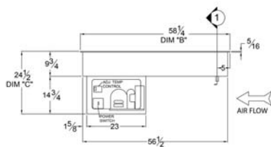
ELEVATION "A" 1/2" = 1'-0"
