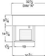
SIDE ELEVATION 1/2" = 1'-0"
