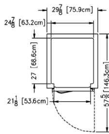
Plan View All Single Section Reach-In Models
