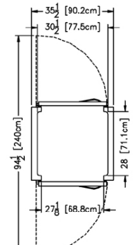
Plan View All Single Section Roll-Thru Models
