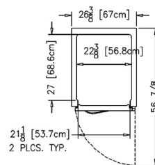
Plan View All Single Section Reach-In Models
