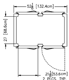
Plan View All Two Section Pass-Thru Models
