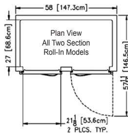
Plan View All Two Section Reach-In Models
