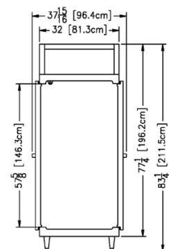
Section View All Pass-Thru Models
