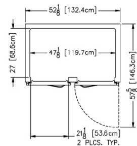
Plan View All Two Section Reach-In Models
