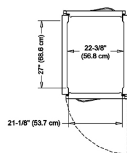
Plan View All Single Section Pass-Thru Models
