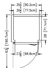
Plan View All Single Section Roll-In Models
