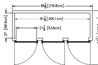
Plan - R/AHT332WUT
