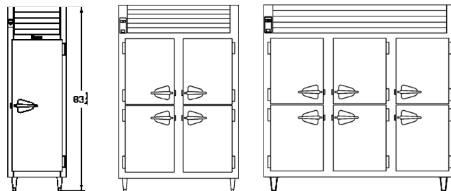
Section - All Models
