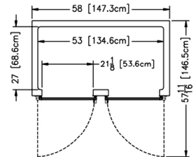
Plan - R/AHT232WUT
