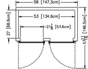
Plan - R/AHT232WUT
