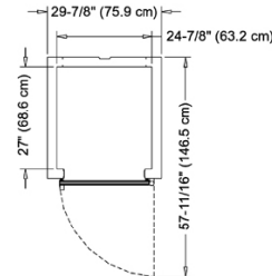
Plan - R/AHT132WUT
