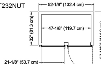
Plan - R/AHT232NUT
