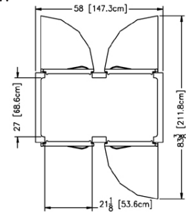
Plan - R/AHF232WP
