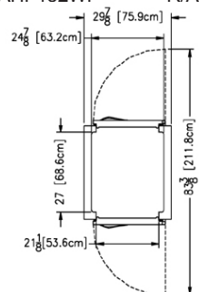
Plan - R/AHF132WP
