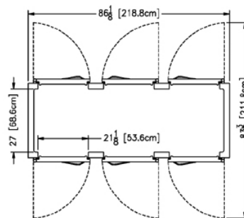
Plan - R/AHF332WP
