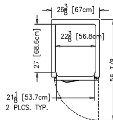
Plan View All Single Section Reach-In Models
