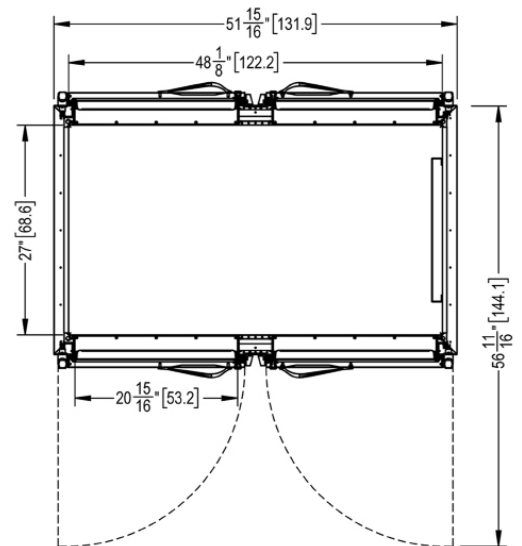
G26014P Non Control Side Glass Door Hinged Left-Right Shown (other door combinations & hinging available)
