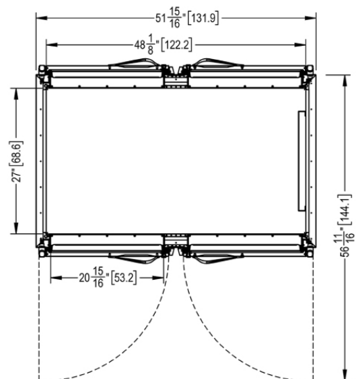
G26004P Non Control Side Glass Door Hinged Left-Right Shown (other door combinations & hinging available)
