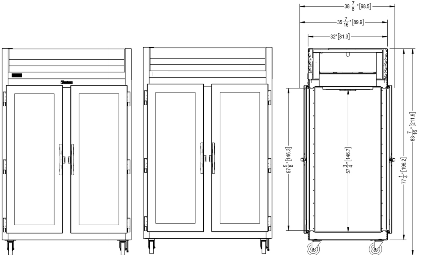
G21014P Control Side Hinged Left-Right Shown (other hinging available)
