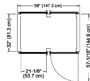
Plan - R/AHT232WP/UT
