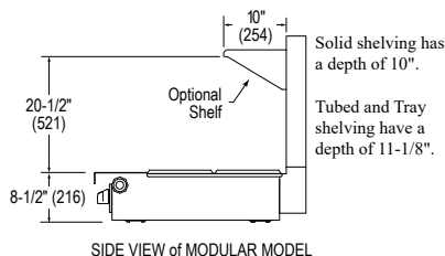
SIDE VIEW of MODULAR MODEL
