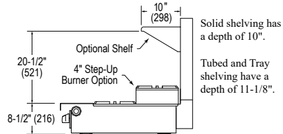
SIDE VIEW of MODULAR MODEL
