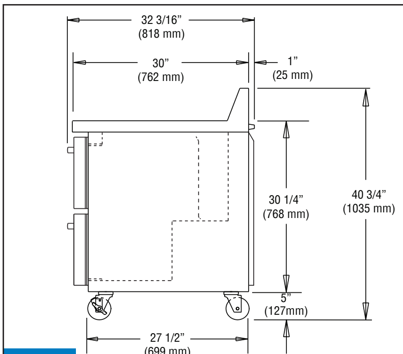
SIDE VIEW
