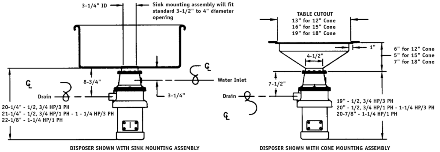
DISPOSER SHOWN WITH SINK MOUNTING ASSEMBLY
