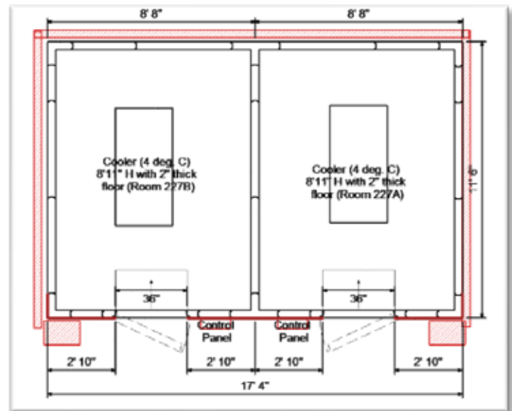
Construction Diagram
