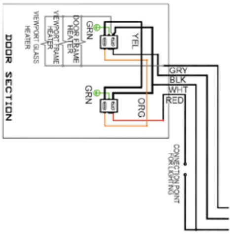
STANDARD SINGLE DOOR W/ EXT. & INT. SWITCHES
