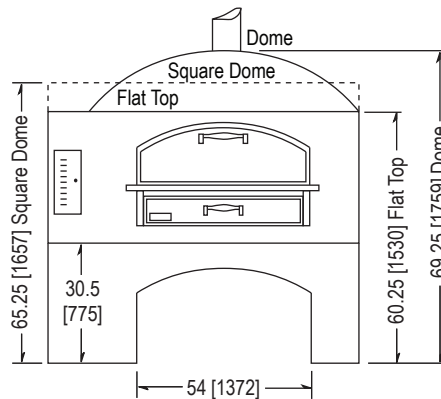
SINGLE OVEN FRONT VIEW
