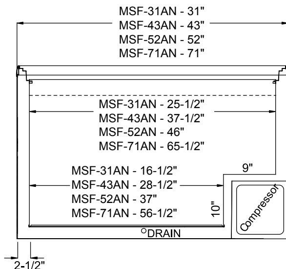
ELEVATION VIEW
