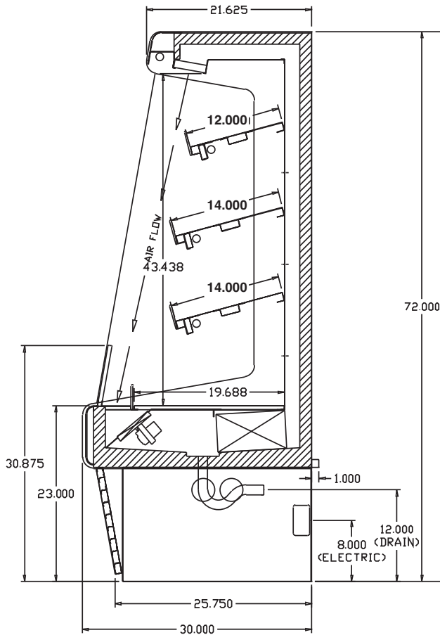
Cross Section
