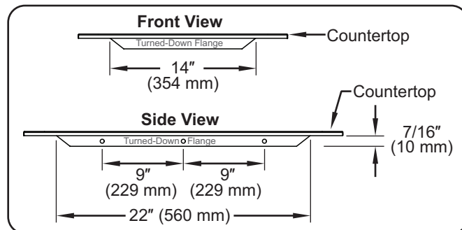
Flanged Countertop Installation Dimensions
