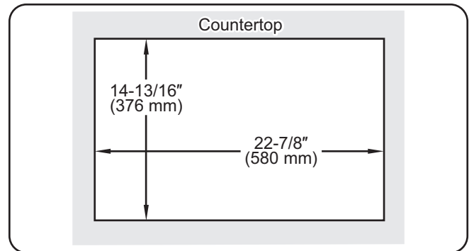
Countertop Cutout
