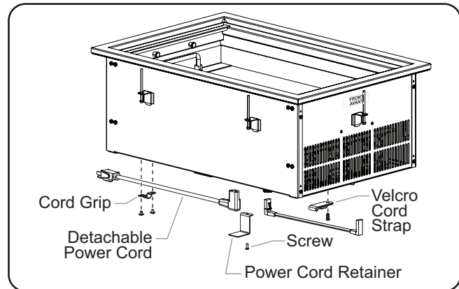
Installing the Detachable Power Cord and Retainer
