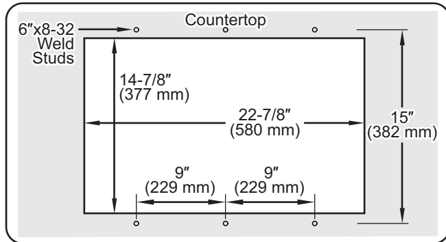
Mounting Stud Installation Dimensions
