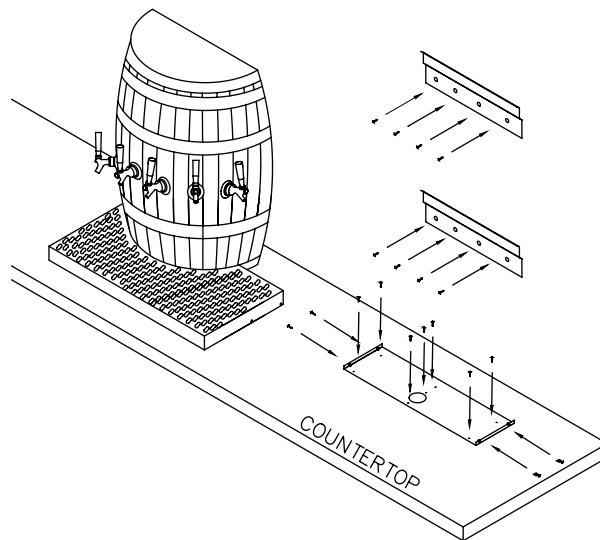
MOUNTING DETAILS
