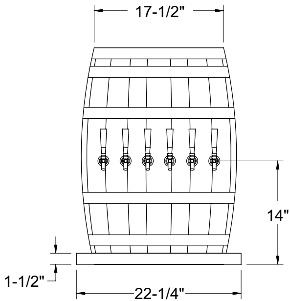
FRONT ELEVATION
