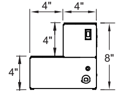
SIDE VIEW (IF POWERCORD RIGHT)
