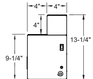
SIDE VIEW (IF POWERCORD RIGHT)
