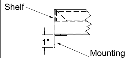
Wall Mounting Bracket
