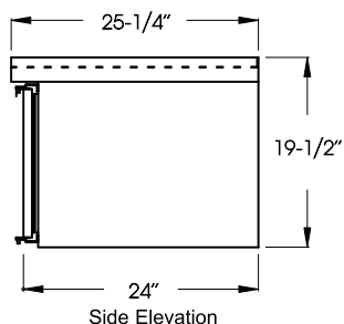
Side Elevation
