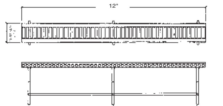
Roller Conveyor
