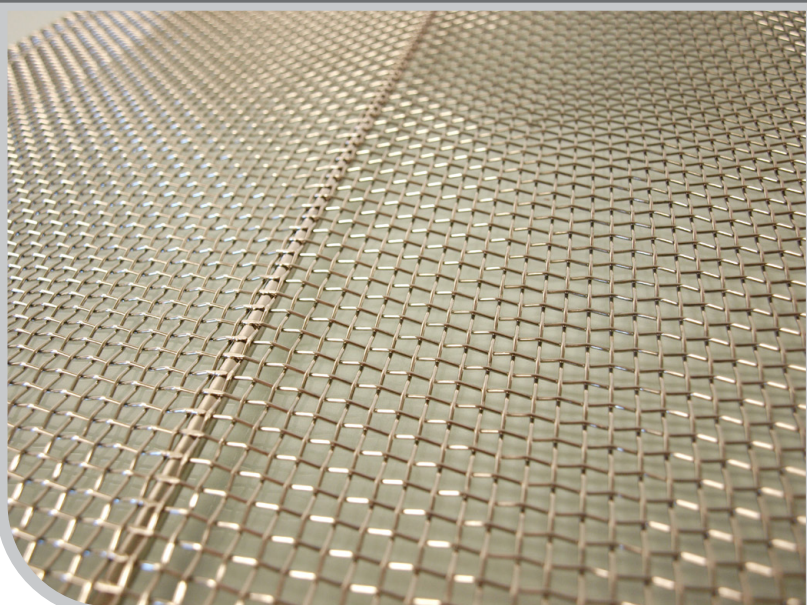
17" x 25" Screen Part # 618-0007A for 618L, 718L fryers
