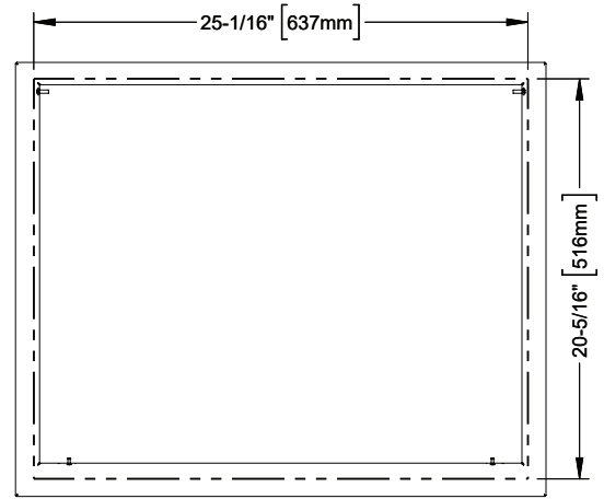
CUT-OUT DIMENSIONS
