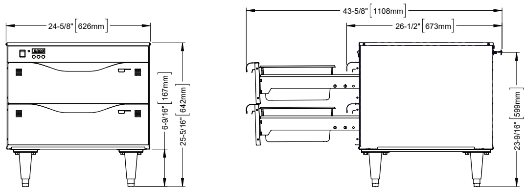
Shown with 6" [152mm] legs
