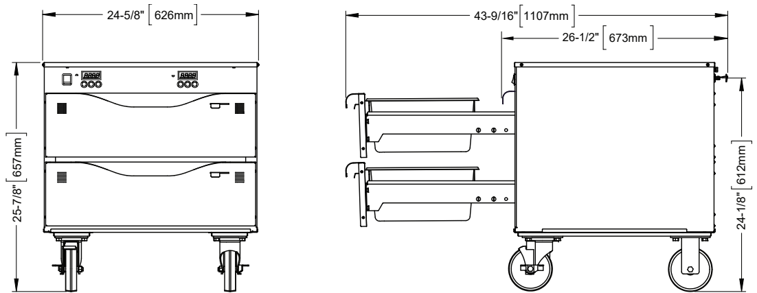
Shown with 5" [127mm] casters
