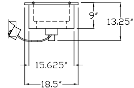
9560xN-Z END VIEW
